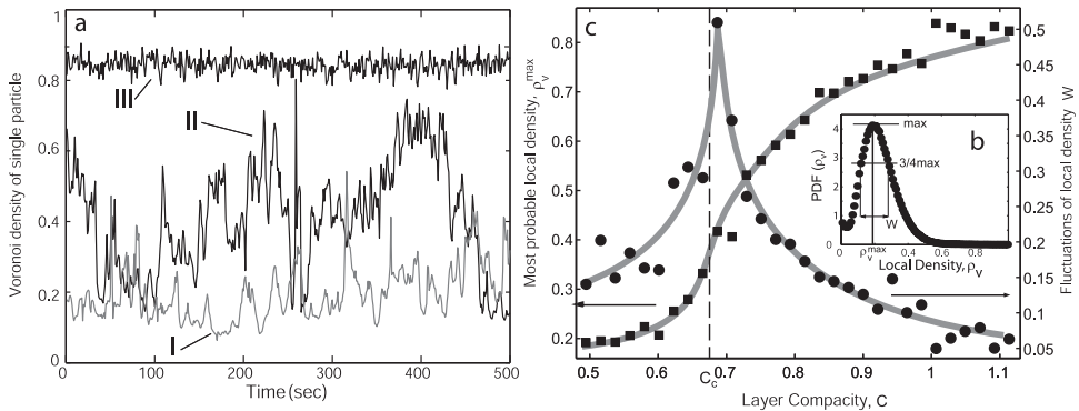
Fig. 4 – Local density. a) Time series of the local densities for a typical individual sphere, illustrating the characteristic fluctuations, for the binary gas ( C = 0.578 , trace I), segregation liquid ( C = 0.687 , just above C_c , trace II), and segregation crystal ( C = 1.071 , trace III) phases. Inset b): for each value of C data, 750000 particle positions were used to construct a PDF for the local density. c) From this PDF ( \rho_v ) we extract the characteristic, i.e. most probable, local density, \rho_v^{\max} (squares) and the width gives an estimate of the microscopic fluctuations, w (circles). The dashed line is drawn at the critical compaction value, C_c , measured in ref. [16] and the solid grey lines are guides to the eye.
