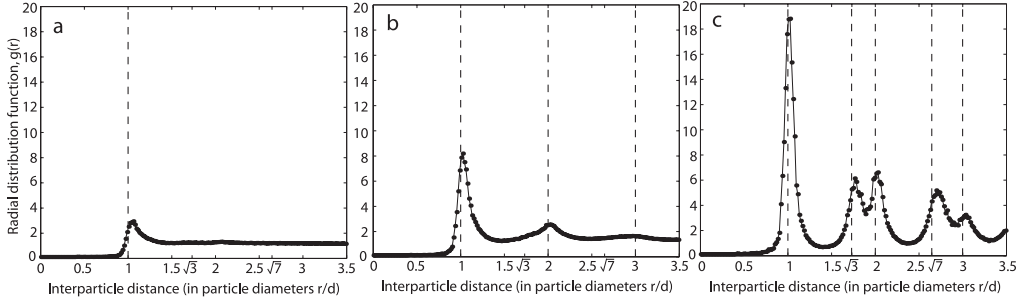
Fig. 3 – Radial distribution functions, g(r) , for states in each of the segregation phases: a) binary gas ( C = 0.516 ), b) segregation liquid ( C = 0.729 ) and c) segregation crystal ( C = 1.071 ). The vertical dashed lines correspond to the expected location of the peaks in each of the segregation phases. Note that the image processing and finite pixel size of the camera “blur” the distributions slightly, which accounts for the non-zero value of g(r) , for r < d .
