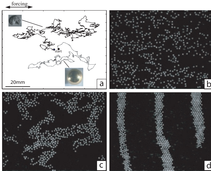
Fig. 1 – a) Stochastic trajectories taken over a period of 1 min for a single particle on the tray. The black and grey trajectories (poppy seed and phosphor-bronze sphere, respectively) show two quasi-random walks on the oscillating surface. The distributions of step lengths are exponential (poppy seeds) and Gaussian (spheres) [15]. The three photographs correspond to states within the various phases: b) binary gas ( C = 0.516 ), c) segregation liquid ( C = 0.729 ) and d) segregation crystal ( C = 1.071 ). The binary layer was started from mixed initial conditions in each case and frames were taken after 3 min of shaking so that a (macroscopic) quasi-steady state was achieved. Note that only the phosphor-bronze spheres are visible.
