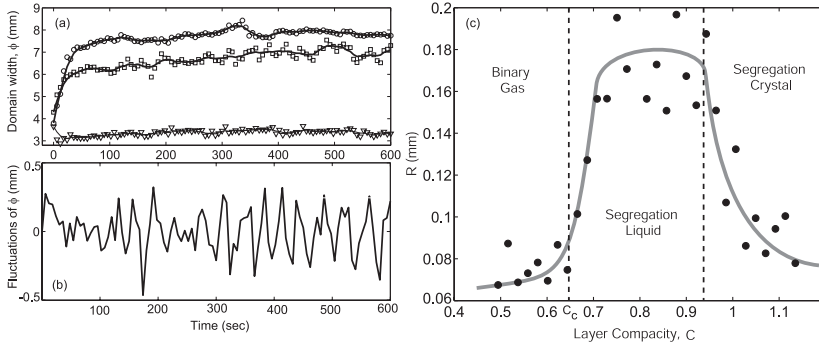
Fig. 2 – a) Time series of \phi(t) : \nabla for C = 0.580 , \square for C = 0.751 and \circ for C = 1.028 . We filtered \phi(t) through a digital low-pass finite impulse response (FIR) digital filter algorithm with brickwall at \omega = 2.29 \times 10^{-3} Hz and -3 dB point at \omega = 9.78 \times 10^{-3} Hz to obtain \phi_{\text{filtered}}(t) (solid curves). b) Time series of the macroscopic fluctuations, f(t) = \phi(t) - \phi_{\text{filtered}}(t) for C = 0.751 . c) Root mean square of the fluctuations, R , plotted as a function of C . The dashed line at C_c = 0.647 denotes the binary-gas-segregation-liquid transition point C_c measured in ref. [16]. The dashed line at C = 0.943 is a guide to the eye for the possible location of the segregation liquid to crystal transition. The solid grey line is a guide to the eye.
