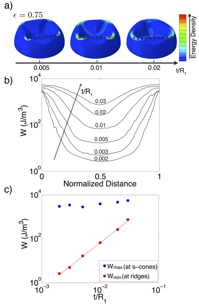
Fig. 6 The effect of shell thickness. (a) Snapshots of shells with increasing t/R_1 ratios at \epsilon = 0.75 , under point indentation. The color map indicates strain energy density. The black dashed lines trace a path along ridges between adjacent s-cones. (b) Strain energy density, W , along the paths in (a), for shells with thickness to radius ratio in the range 0.002 < t/R_1 < 0.03 , indented to \epsilon = 0.75 under point indentation. (c) W_{\max} (at the s-cones) and W_{\min} (at the ridges), as a function of t/R_1 . The solid red line indicates a power-law fit to the data, with exponent 2.1 \pm 0.1 .
